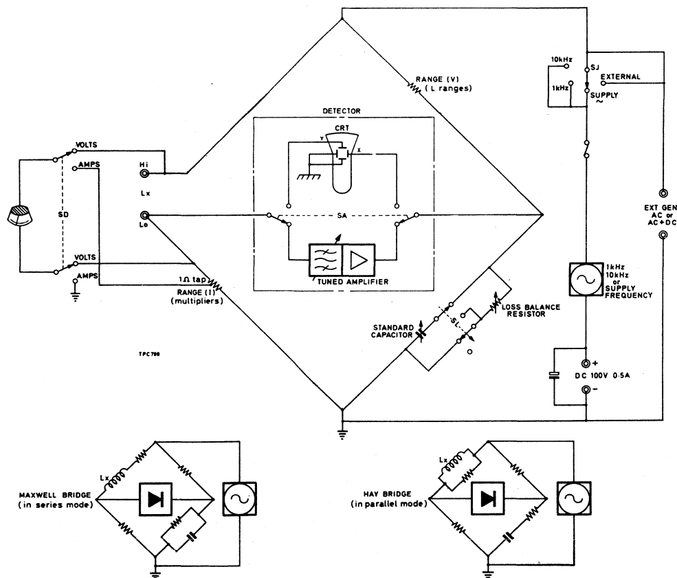
Functional diagram
