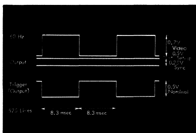
Waveform for I.f. response measurement
