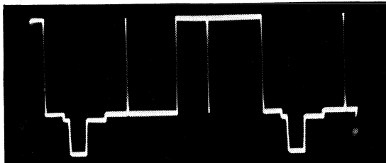
525 line Monochrome Waveform TF 2905/9
