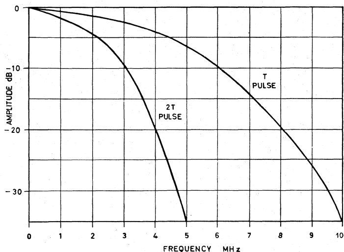
Fig. 2. Spectrum of a sine-squared pulse.
