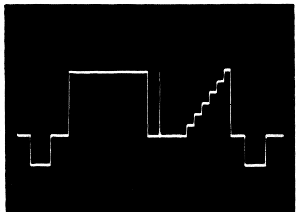
Fig. 10. Monochrome insertion signal for 625 lines.
