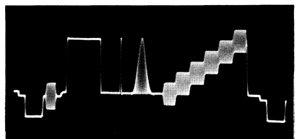
Colour test signal for 525-line systems
