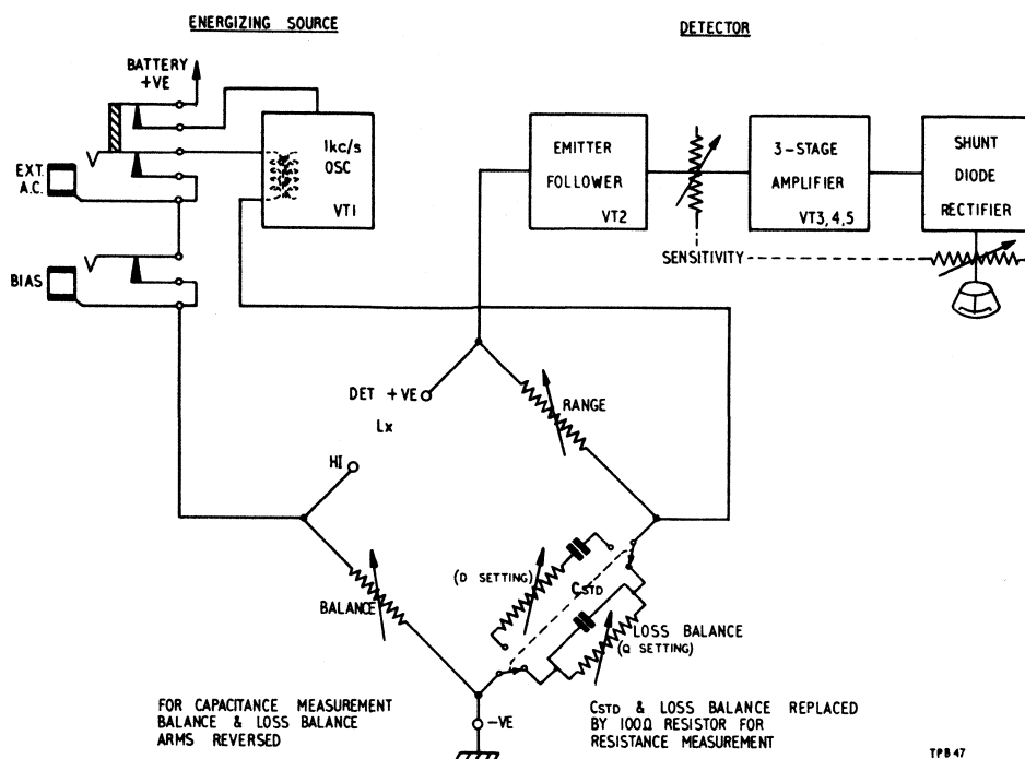
Functional Diagram for A.C. Measurements
