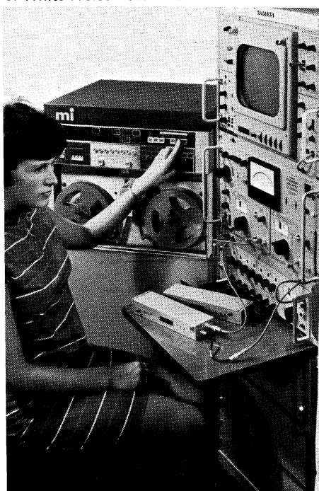
The "Autotest" response measuring system incorporating Siemens programmable instrumentation in use at the St. Albans factory of Marconi Instruments to check out filters from the large scale production of White Noise Test Sets.
