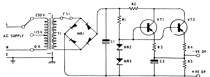
TM 9808 CIRCUIT DIAGRAM
