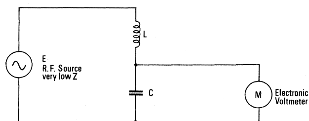
Fig. 4 Functional arrangement of circuit magnification meter.
