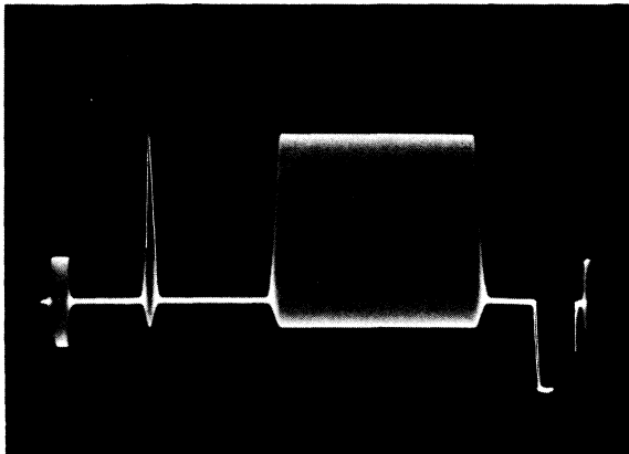
Fig. 8. Gain inequality indicated by combined luminance and chrominance sine squared pulse and bar.
