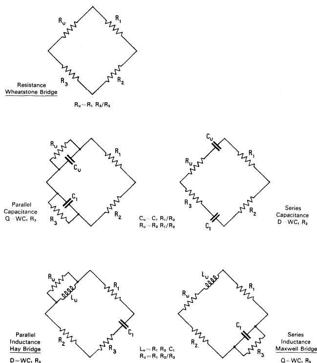
Fig. 1 Impedance-ratio-arm bridges.
