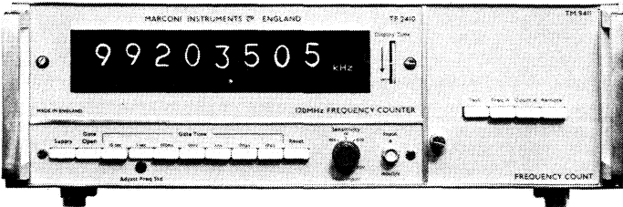
TF 2410 with plug-in Frequency Count Module TM 9411.
