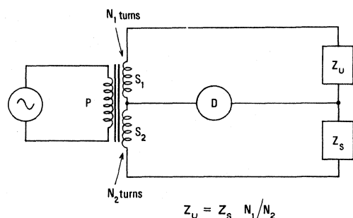
Fig. 2 Transformer-ratio-arm bridge.
