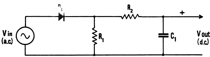
Fig. 1 Average Detector.
