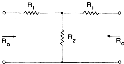
T Network
